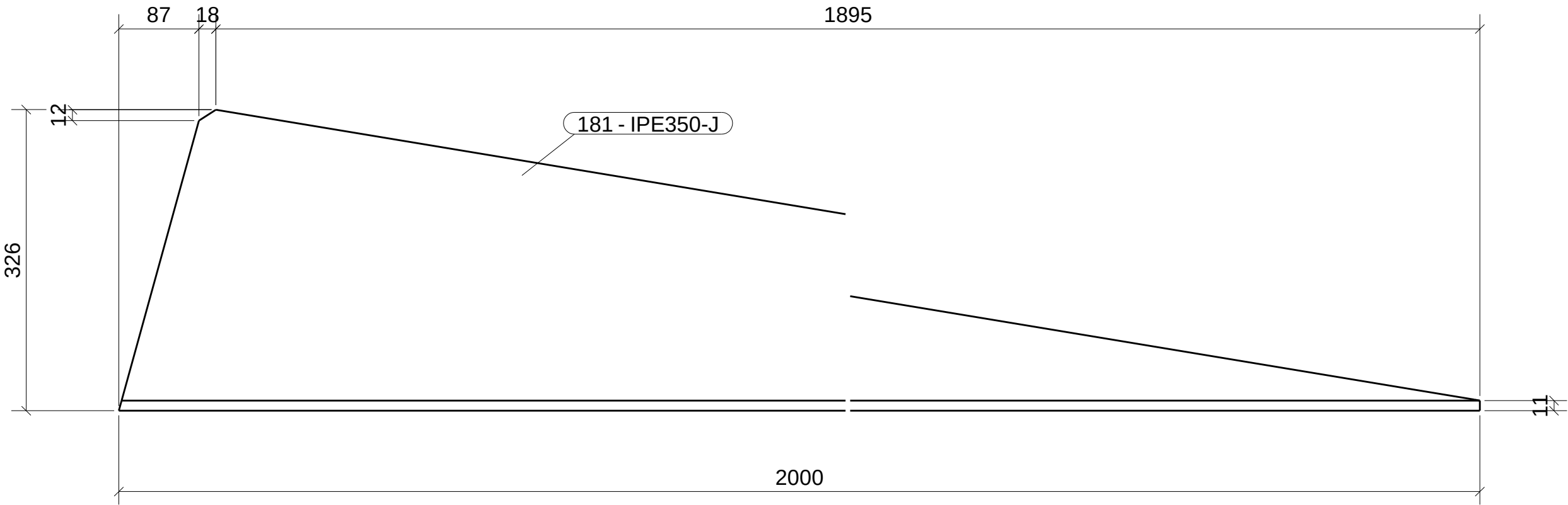
FRONT VIEW
